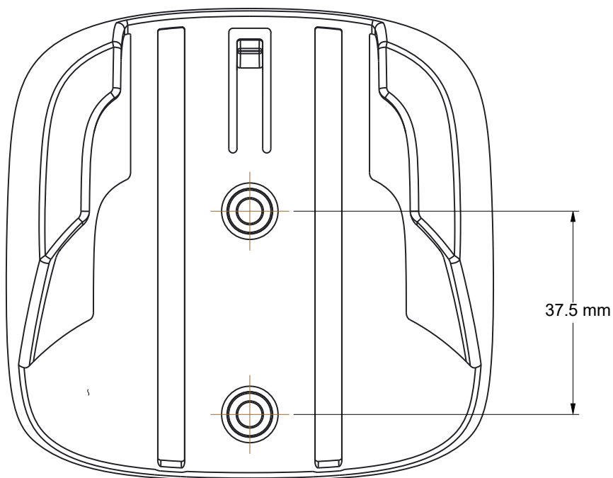
Figure 1-9 Desk Mount Bracket Template
