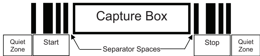
Figure I-2 CapCode Structure
