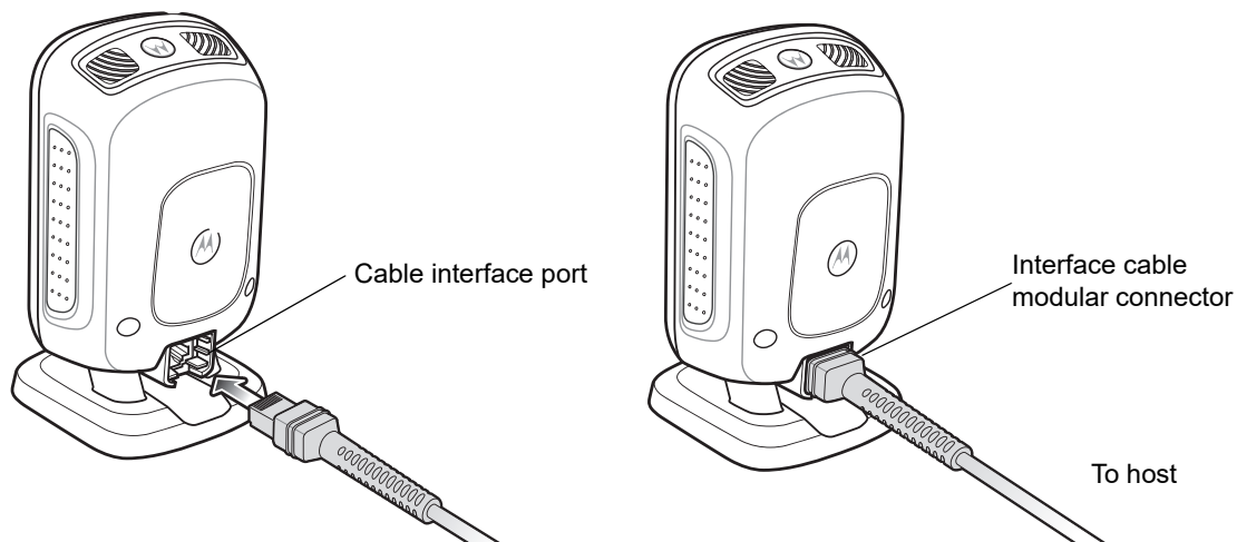
Figure 1-2 Installing the Cable
