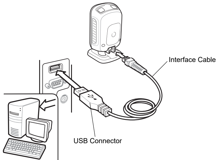
Figure 6-1 USB Connection
