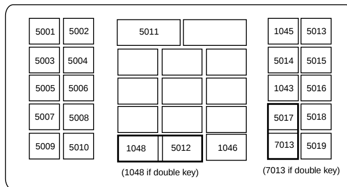
Figure 5-3. NCR 7052 32-KEY
